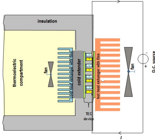
Figure 2: Schematic of the TER unit.
