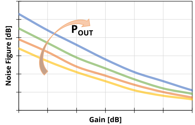
Fig. 3. Qualitative example of Noise Figure-vs-Gain and P_{\text{out}} curves of an amplifier.
