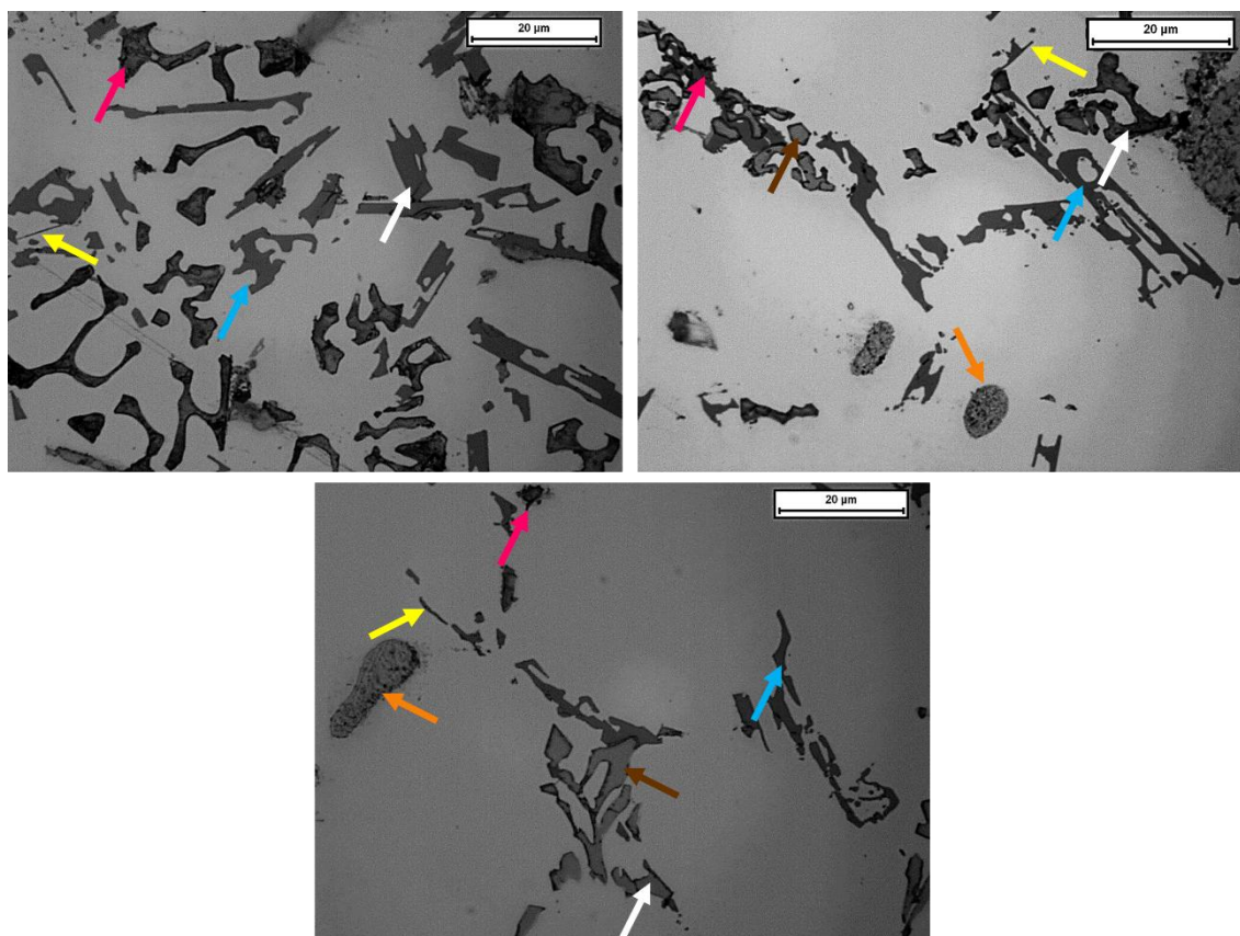
Figure 3. Optical microscope images of alloy EN AC 45300 (100x magnification, marker 20 \mu m). Microstructures and intermetallic phases. Blue = Eutectic silicon; purple = Mg-based phase; white = Q-phase; brown = \alpha -Fe; yellow = \beta -Fe; orange = Al-Al 2 Cu-Si.
