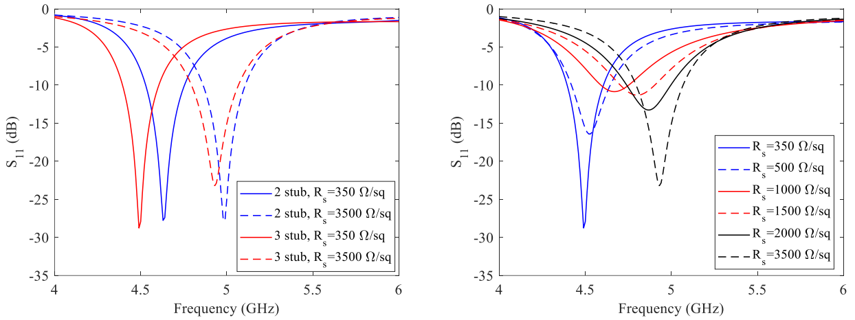
Fig. 3. Comparison of the return loss of the two stub antenna with the three stub antenna.
