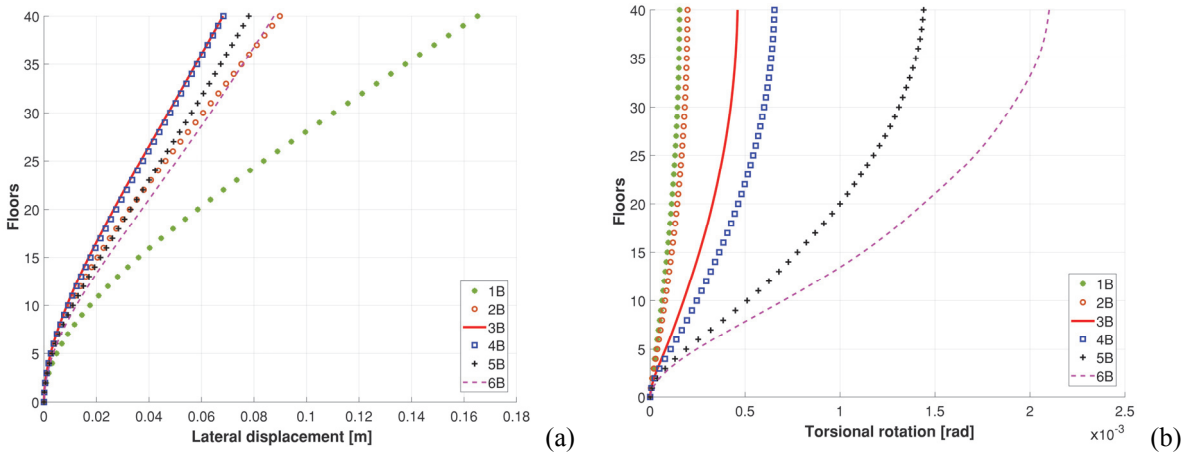
Fig. 3. Diagrid tube coupled with open-section shear wall: (a) lateral displacements, (b) torsional rotations.
