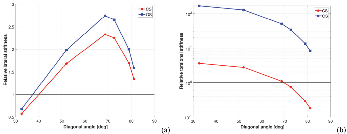
Fig. 5. Relative stiffness of diagrid and shear wall: (a) lateral stiffness, (b) torsional stiffness.
