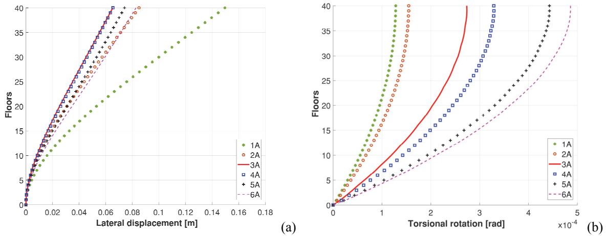
Fig. 2. Diagrid tube coupled with closed-section shear wall: (a) lateral displacements, (b) torsional rotations.
