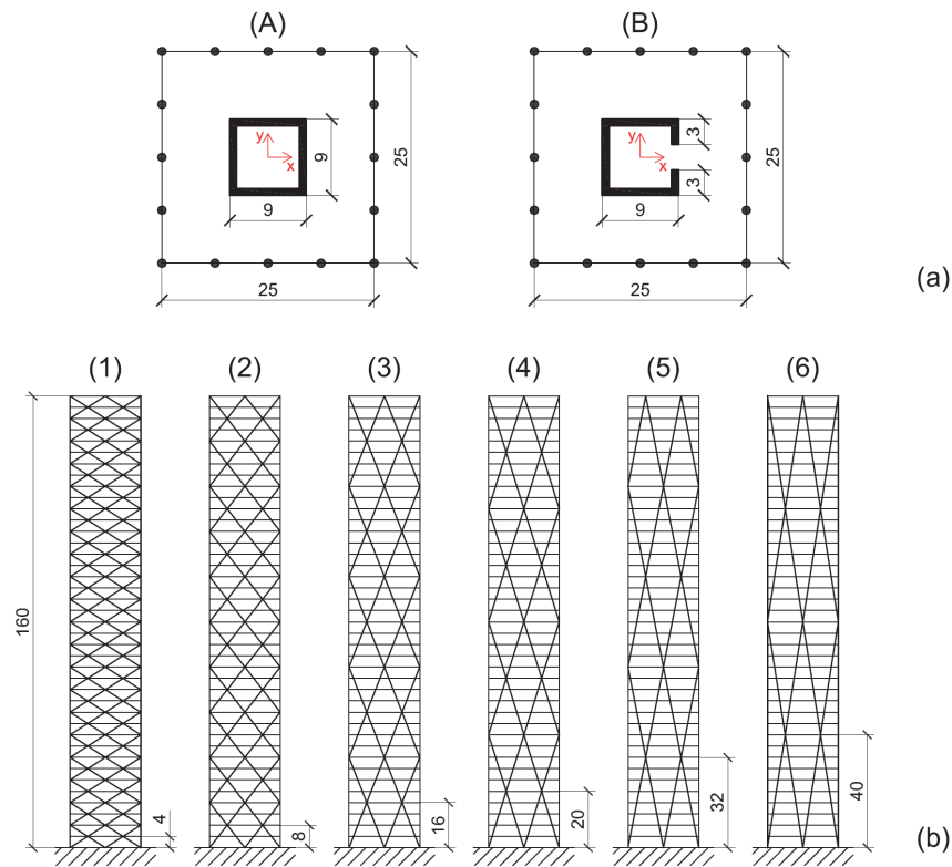
Fig. 1. Building geometry: (a) floor plans, (b) lateral views.
