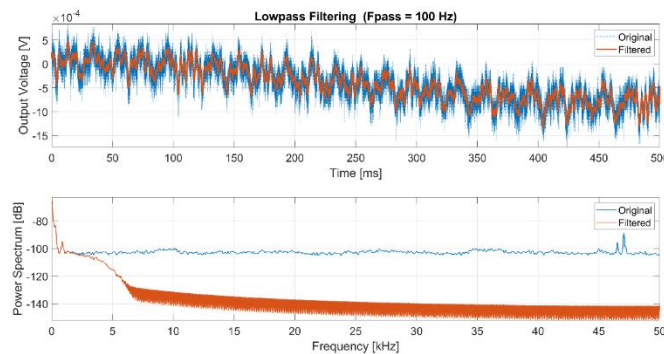
Figure 42: Low-pass filter at exciting frequency applied to an example of the acquisition data sets at 100 Hz.
