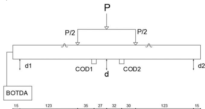
Figure 5. LVDT arrangement.
