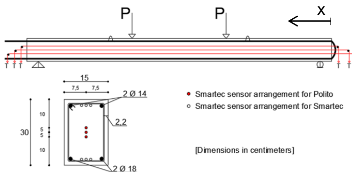
Figure 3. Sensors positioning.
