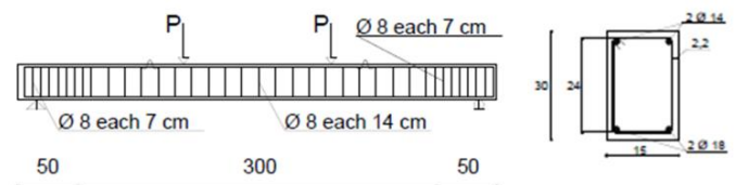
Figure 1. Reinforced Concrete beam details.
