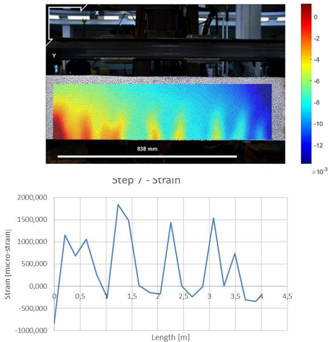
Figure 18. Comparison between FOS and DIC.
