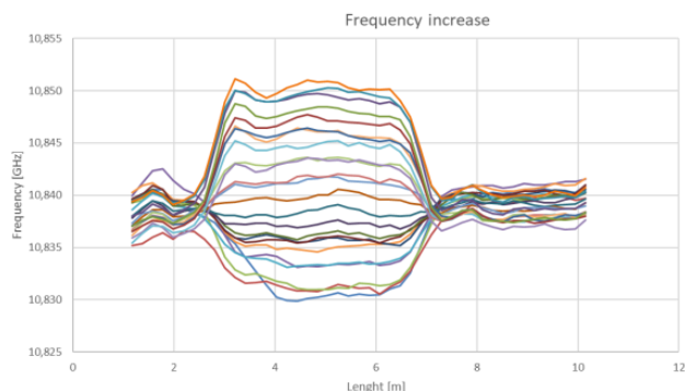
Figure 8. Brillouin frequency change.
