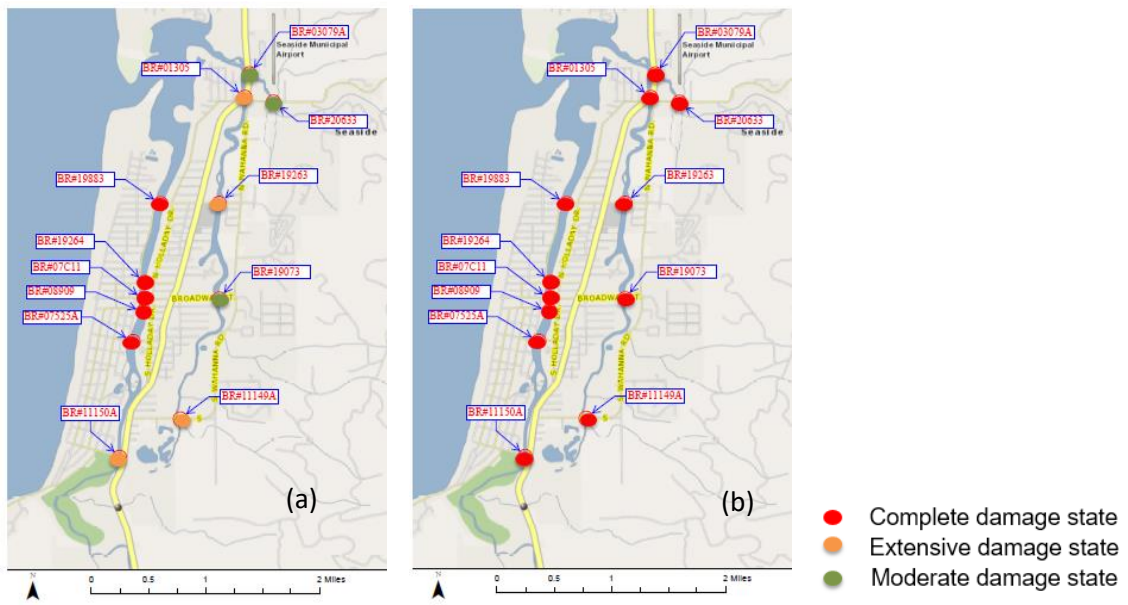
Figure 6. Damage to lifelines components: highway bridges in Seaside. Tsunami-only scenario (a) and Earthquake & tsunami scenario (b).
