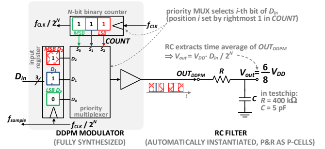
Fig. 9. DDPM DAC architecture, comprising a digital block generating the DDPM sequence and a 1 st -order RC filter extracting the DC value of its output voltage.
