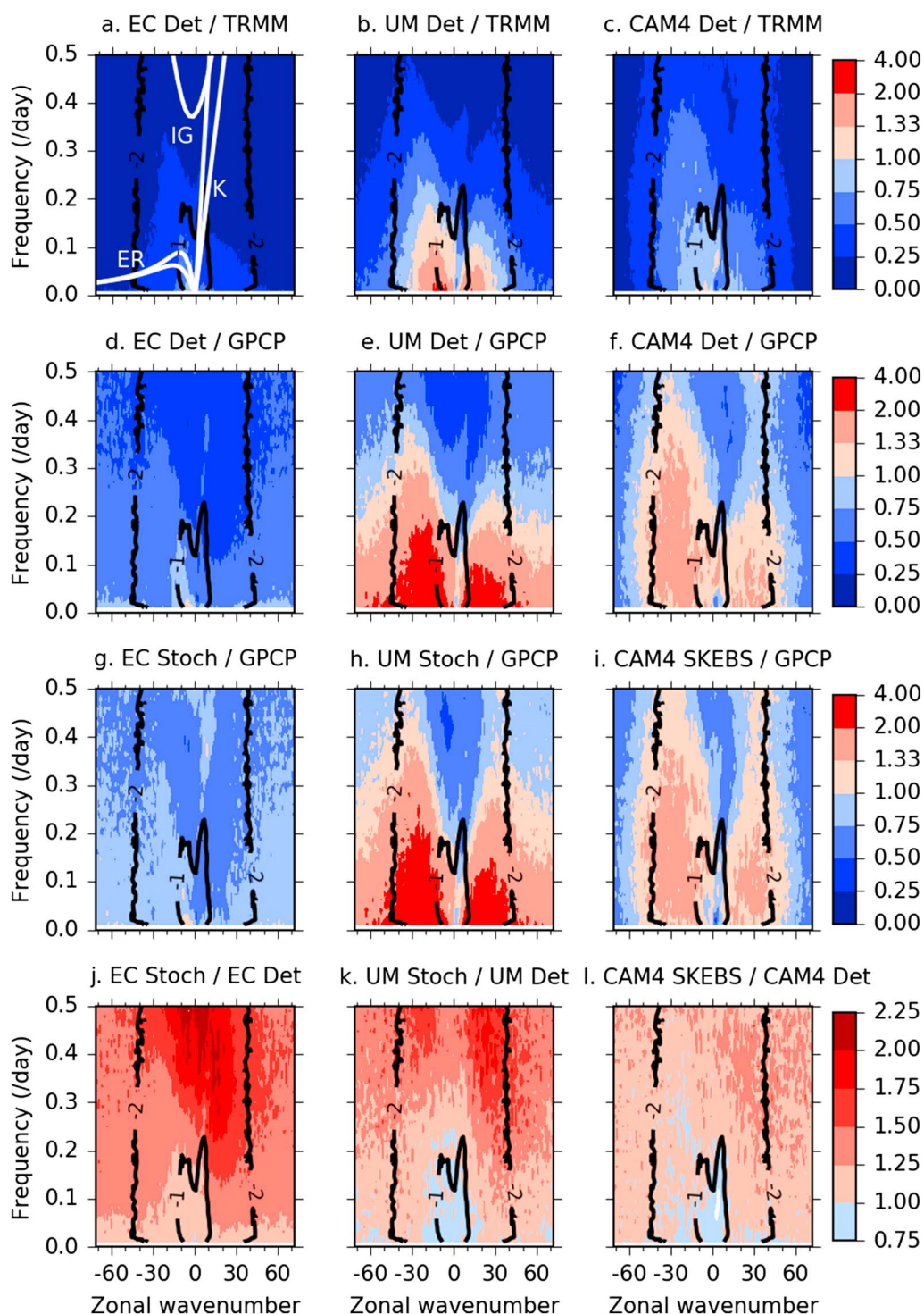
Figure 5. Filled contours show ratios between different data sets of the spectral power of precipitation in meridionally symmetric equatorial wave modes averaged between 15^{\circ}\text{S} – 15^{\circ}\text{N} as a function of zonal wave number and frequency. Results relating (a, d, g, and j) to the low-resolution EC-Earth configurations, (b, e, h, and k) to the low-resolution UM configurations, and (c, f, i, and l) to the CAM4 Det and SKEBS configurations. Figures 5a–5c show the ratio of power in the deterministic configurations to that in TRMM, Figures 5d–5f the ratio of power in the deterministic configurations to that in GPCP, Figures 5g–5i the ratio of power in the stochastic configurations to that in GPCP, and Figures 5j–5l the ratio of the power in the stochastic configurations to that in the deterministic configurations. White lines in Figure 5a indicate theoretical dispersion curves for Kelvin waves (K), wave number 1 inertia gravity waves (IG), and equatorial Rossby waves (ER) with equivalent depths 12 m and 50 m. Stochastic physics is effective at increasing the power and reducing the model biases at high frequencies in EC-Earth and the UM, with SKEBS in CAM4 having a smaller effect.
