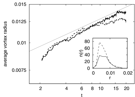
FIG. 4. Average vortex radius as a function of time, starting from random initial conditions, when only small-scale dissipation is present (solid line) and when a large-scale energy sink is also included (dashed line). The dotted line shows the prediction of the scaling theory of Carnevale et al. [26]. The inset shows the histogram of the vortex radii at time t = 15 without (solid line) and with (dashed line) the large-scale energy sink.
