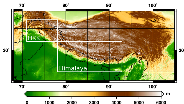
FIG. 1. Orography of the HKKH area (DEM from the GLOBE project). The white boxes represent the HKK and the Himalaya subregions considered in this study.
