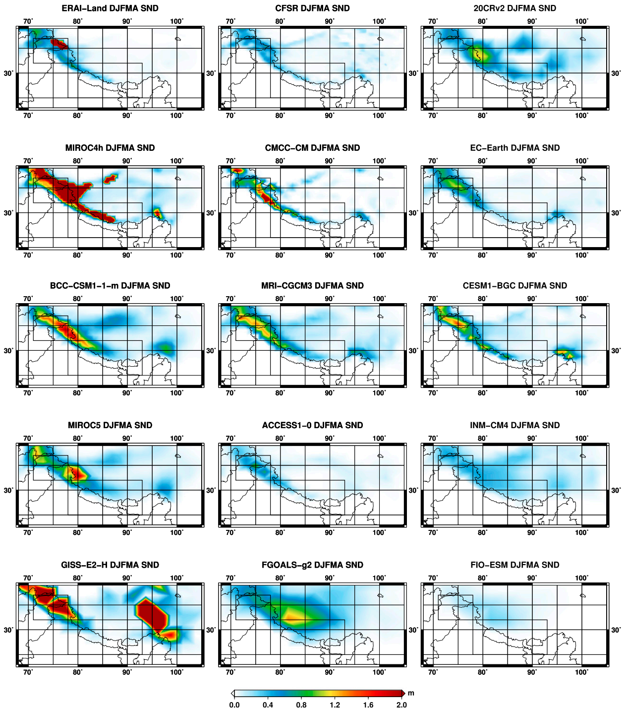
FIG. 2. Spatial distribution of the mean winter (DJFMA) SND for (top row) ERA-Interim/Land, CFSR, 20CRv2, and (other rows) a set of CMIP5 GCMs. The maps represent multiannual means over the period 1980–2005. Reanalyses and models are ordered by decreasing spatial resolution. The boxes highlight the HKK (west) and Himalaya (east) subregions considered in this study.
