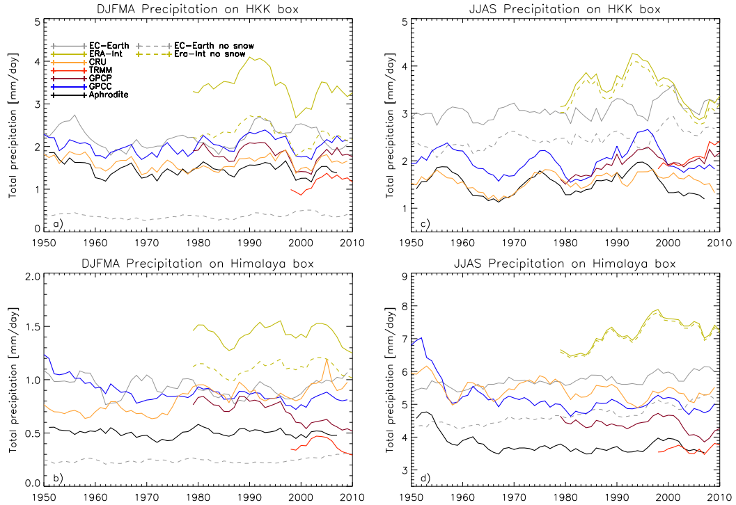
Figure 8. Same as Figure 7, after filtering the time series with a 5 years running mean.
