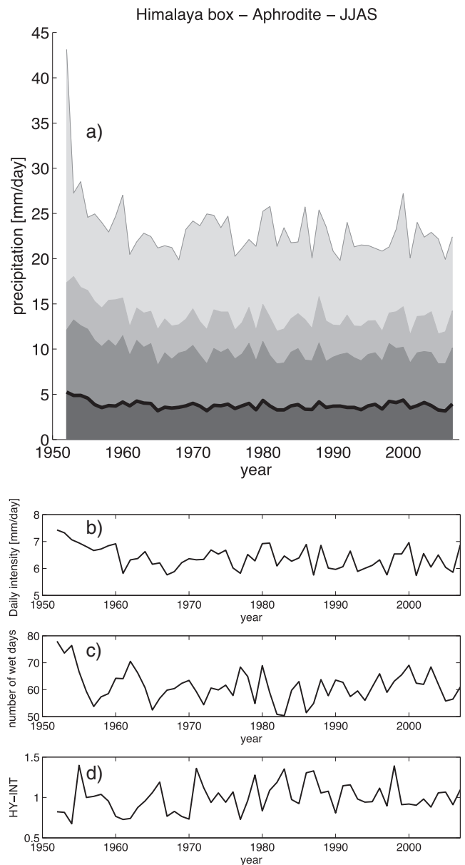
Figure 10. Precipitation statistics for APHRODITE in the Himalaya domain during summer. Time series of (a) average daily precipitation (black thick line) and precipitation above the 90th, 95th, and 99th percentiles (shaded regions); (b) daily precipitation intensity; (c) number of days with precipitation larger than 1 \text{ mm d}^{-1} (wet days); and (d) the hydroclimatic index HY-INT.
