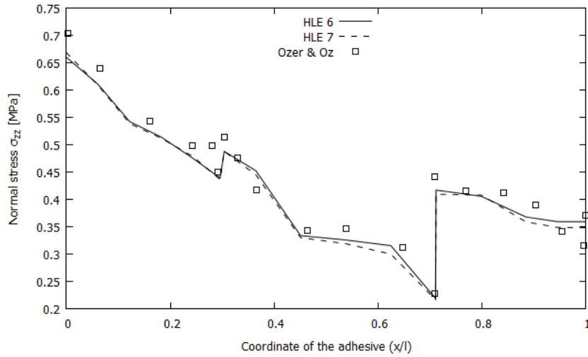
Figure 10: Peel Stress along x-axis.
