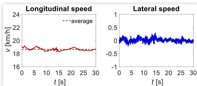
FIGURE 6 Longitudinal and lateral speeds (test on STEVE vehicle at 20 km/h on the asphalted road).
