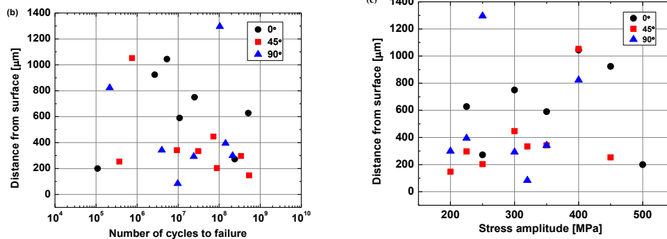
145 Fig. 12 Schematic drawing of distance of defect site from surface (a); and the distance 146 147 from surface versus number of cycles to failure (b) and stress amplitude (c). 148 149 150 151 152 153 154 155 156 157 158 159 160 161 162 163 164 165
