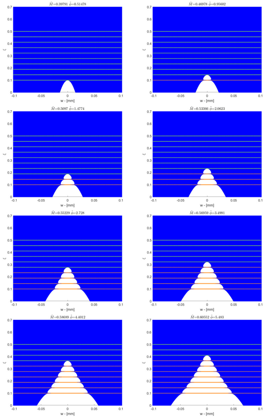
Fig. 3. Concrete element with ten fiber reinforcements under cyclic loading: Crack propagation from the first to the last fiber. Green fibers are considered as elastic, whereas orange ones are considered as plastic.
