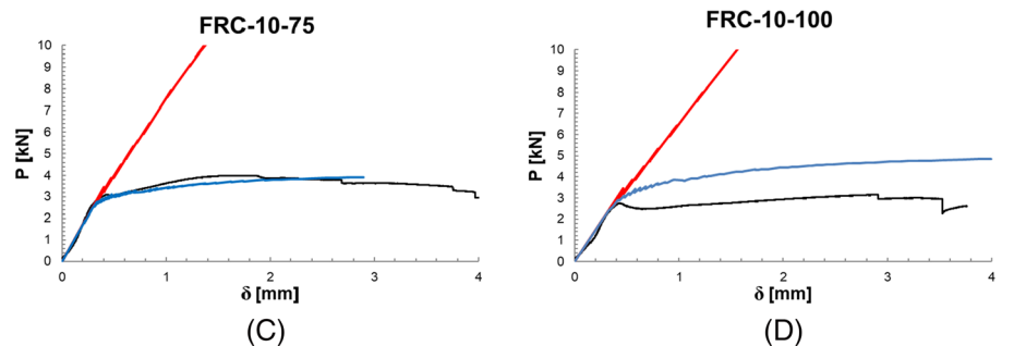
FIGURE 12 Experimental results vs numerical model for the specimen with h = 10 cm. A, FRC-10-04; B, FRC-10-15; C, FRC-10-75; D, FRC-10-100. The red and blue curves are obtained by the numerical model, in the case of yielding and slippage mechanism respectively. The black curve indicates the experimental results
