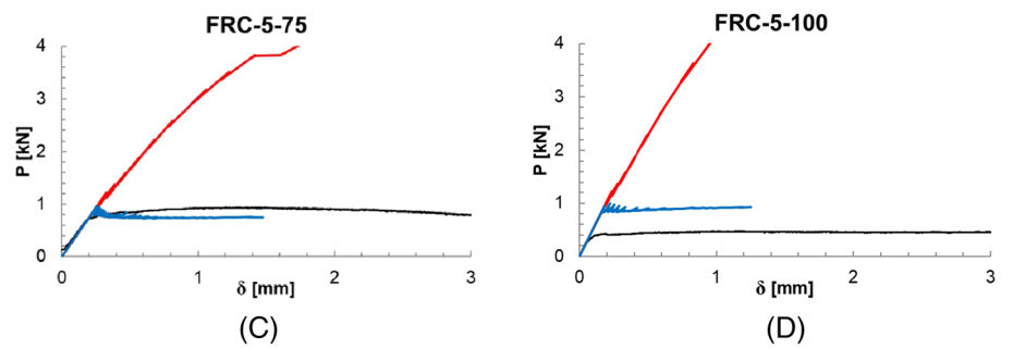
FIGURE 11 Experimental results vs numerical model for the specimen with h = 5 cm. A, FRC-5-04; B, FRC-5-15; C, FRC-5-75; D, FRC-5-100. The red and blue curves are obtained by the numerical model, in the case of yielding and slippage mechanism respectively. The black curve indicates the experimental results
