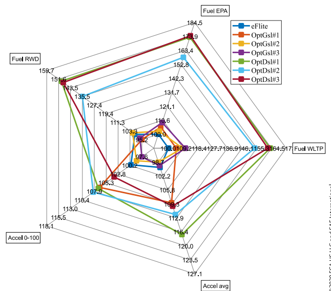
Figure 7. Results for the HEV sizing methodology.
