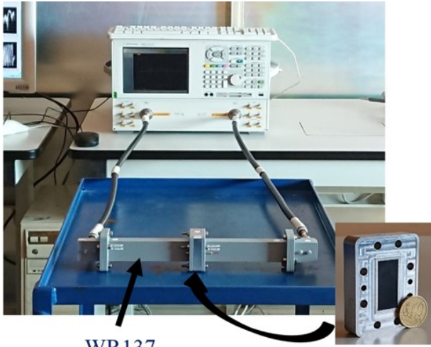
Fig. 4 Waveguide measurements with VNA. See the waveguide spacer in the inset
