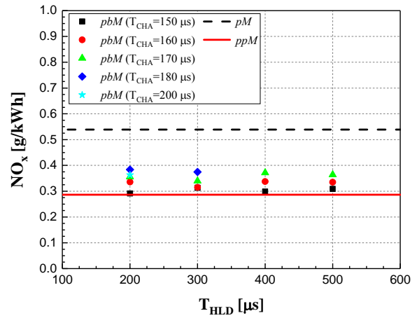
(a) NO_x
