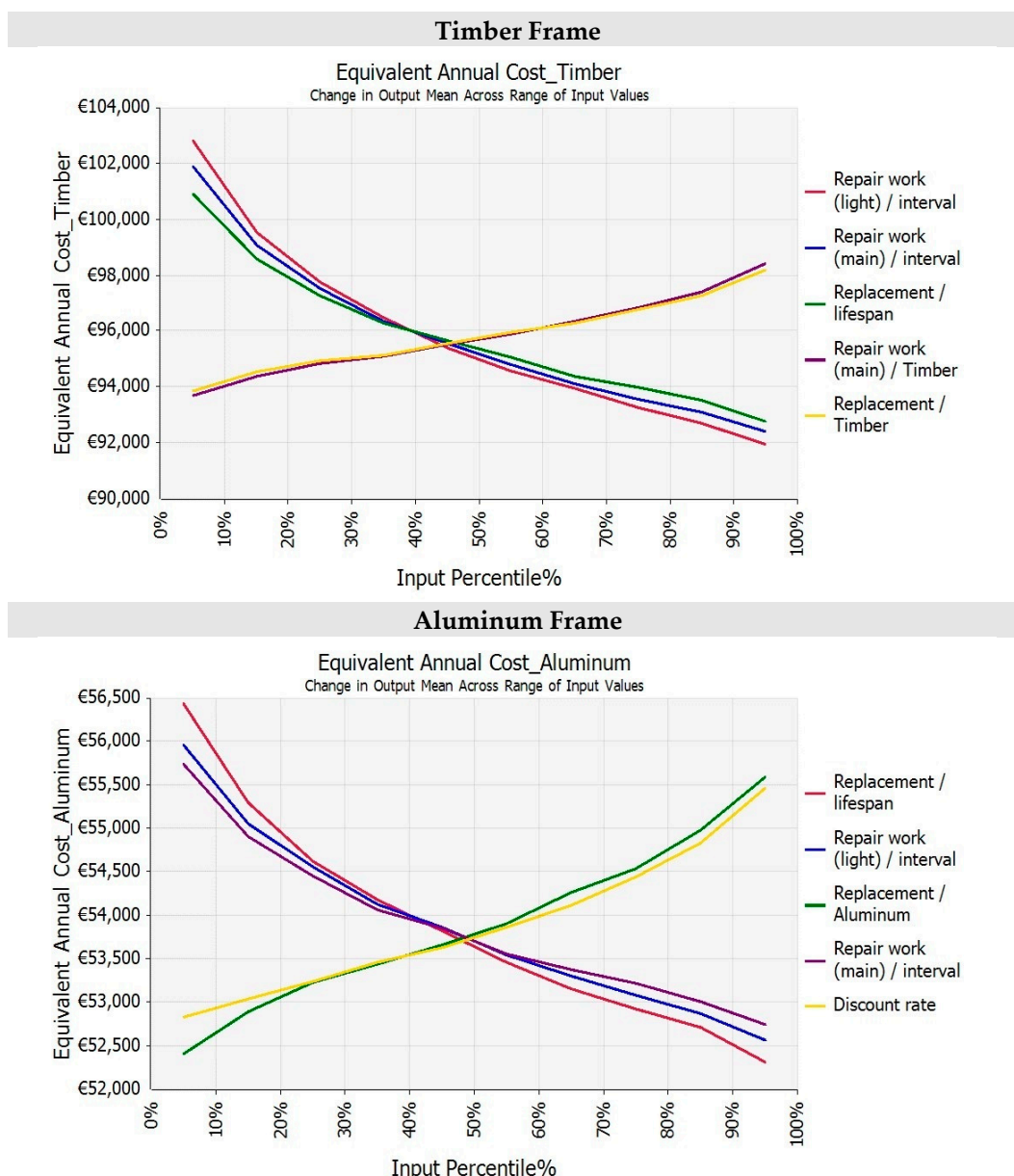
Figure 8. Spider graphs, Timber/Aluminum frames, for stochastic Equivalent Annual Cost. MCM simulation output.
