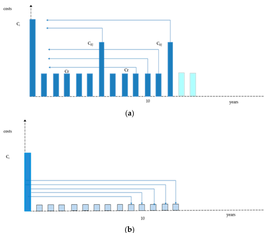
Figure 1. Global Cost discounting schematic example (a) and Annuity Cost annualization schematic example (b).
