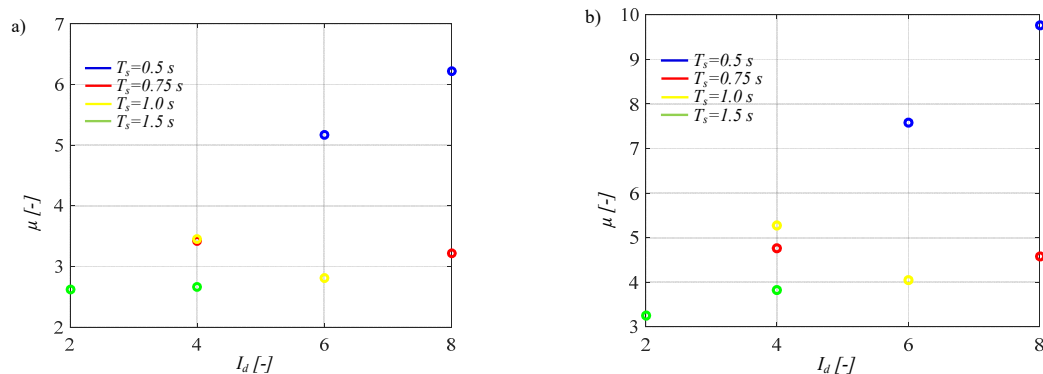
Figure 18. Displacement ductility demand for increasing I_d with fixed T_s and considering \gamma=0.8 , q = 1.5 , for the Chiusaforte site (a) and the Sant’Angelo dei Lombardi site (b).
