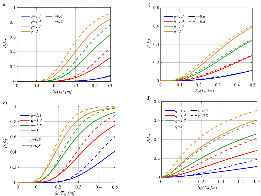
Figure 10. Seismic fragility curves of the superstructure for the Sant' Angelo dei Lombardi site (Italy), related to LS_{\mu,3}=3 , for I_a=2 and T_b=3 s (a), I_a=2 and T_b=6 s (b), I_a=8 and T_b=3 s (c), and I_a=8 and T_b=6 s (d).
