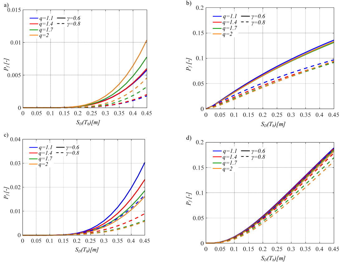
Figure 9. Seismic fragility curves of the FPS for the Chiusaforte site (Italy), related to LS_{b,s}=0.4 m, for I_a=2 and T_b=3 s (a), I_a=2 and T_b=6 s (b), I_a=8 and T_b=3 s (c), and I_a=8 and T_b=6 s (d).
