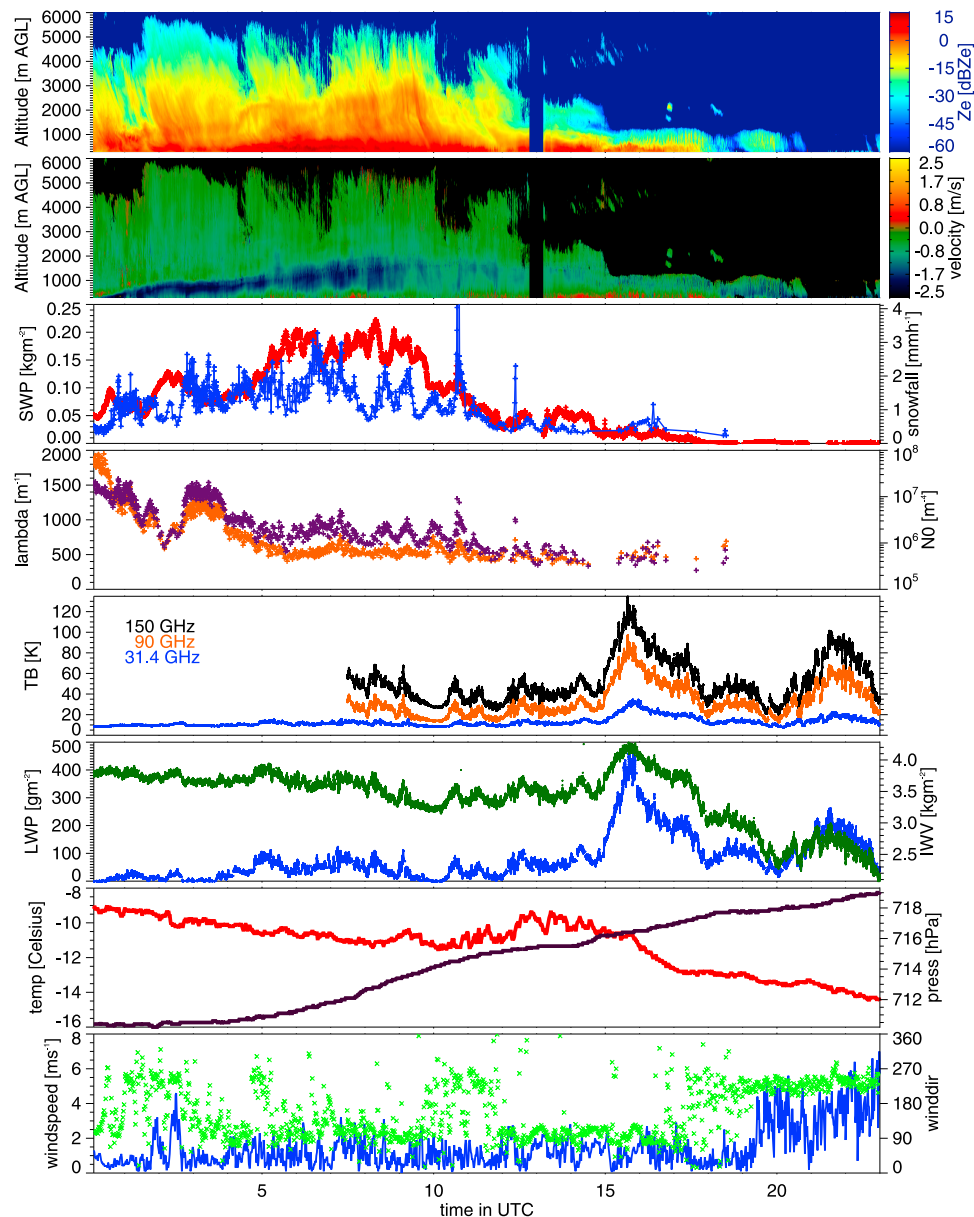
Figure 1. Selected measurements from a strong snow event on 8 February 2009. From the top frame, equivalent K_a -band radar reflectivity in dBZe; radar Doppler velocity in \text{ms}^{-1} (negative values = toward the radar); radar-derived snow water path in \text{kgm}^{-2} (red); 2DVD liquid equivalent snowfall rate in \text{mmh}^{-1} (blue); N_0 in \text{m}^{-4} (orange) and \lambda in \text{m}^{-1} (violet) for exponential snow size distribution (SSD) from 2DVD; MWR brightness temperatures at 150 (black), 90 (orange), and 31.4 (blue) GHz in K; IWP in \text{kgm}^{-2} (green) and LWP in \text{gm}^{-2} (blue) derived from HATPRO; temperature in ^{\circ}\text{C} (red); and air pressure in hPa (black), windspeed in \text{ms}^{-1} (blue), and direction in degree (light green).
