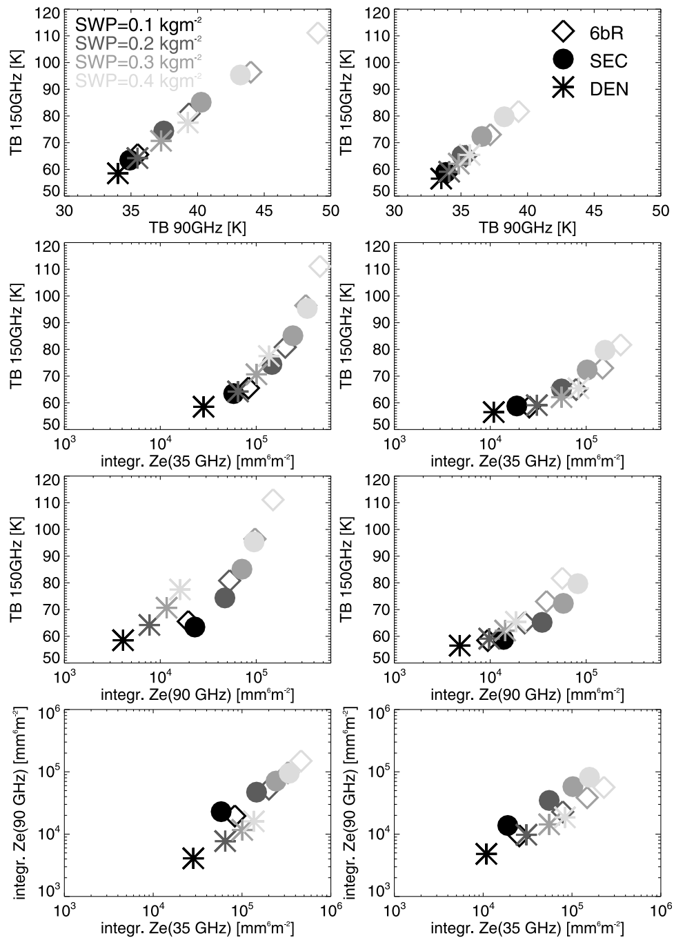
Figure 7. Simulated passive TB in K and vertically integrated radar reflectivity in \text{mm}^6 \text{m}^{-2} factor for a constant atmosphere and different snow microphysics: model results (left) for N_0 = 1 \times 10^6 \text{ m}^{-4} and (right) for N_0 = 1 \times 10^7 \text{ m}^{-4} . The symbols represent different snow habits similar to Figures 5 and 6: 6bR (diamonds), SEC (circles), and DEN (asterisks), whereas the different gray scale illustrates different SWP values ranging from 0.1 to 0.4 \text{kgm}^{-2} . First row: TB at 150 and 90 GHz, second row: TB 150 GHz and integrated Ze at 35 GHz, third row: TB 150 GHz and integrated Ze at 90 GHz, and fourth row: integrated Ze at 90 GHz and 35 GHz.
