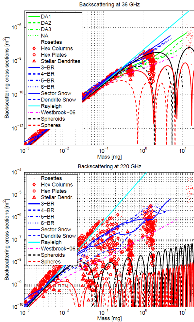
Figure 4. Backscattering cross sections for different habits as a function of ice crystal mass. Results from DDA data sets (Liu, 2008a; Petty and Huang, 2010; Tynnelä et al., 2011), for soft spheres and 0.6 axial ratio spheroids (following the snow densities proposed in Hogan et al. (2012) (dashed) and in Matrosov (2007) (continuous lines)) and the Rayleigh–Gans approximation according to Westbrook et al. (2006) (magenta dash-dotted) have been included.
