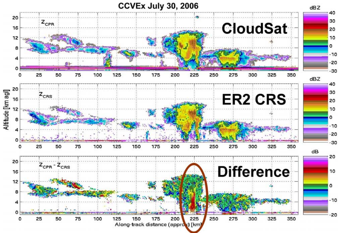
Figure 1. Evidence of multiple-scattering effects from the airborne CloudSat/CALIPSO Validation Experiment (CCVEx). (top) CloudSat radar reflectivity in dBZ ; (middle) ER2-CRS radar reflectivity in dBZ under flying the CloudSat ground track; and (bottom) difference between the CPR and the CRS reflectivities in decibels. This image, courtesy of S. Tanelli (Jet Propulsion Laboratory, California Institute of Technology), was generated using CRS preliminary calibration data courtesy of G. Heymsfield (NASA/GSFC) and L. Li (GEST). Relative calibration between CPR and CRS has been corrected since, and this image should be regarded as calibrated within 3 dB. The MS signature due to the different footprint sizes is evident well beyond this calibration uncertainty.
