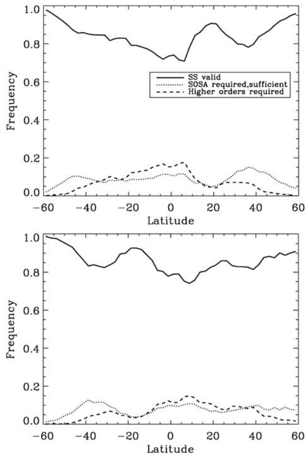
Figure 11. (top) Zonal mean of the data presented in Figure 9. (bottom) Same for the JJA period.
