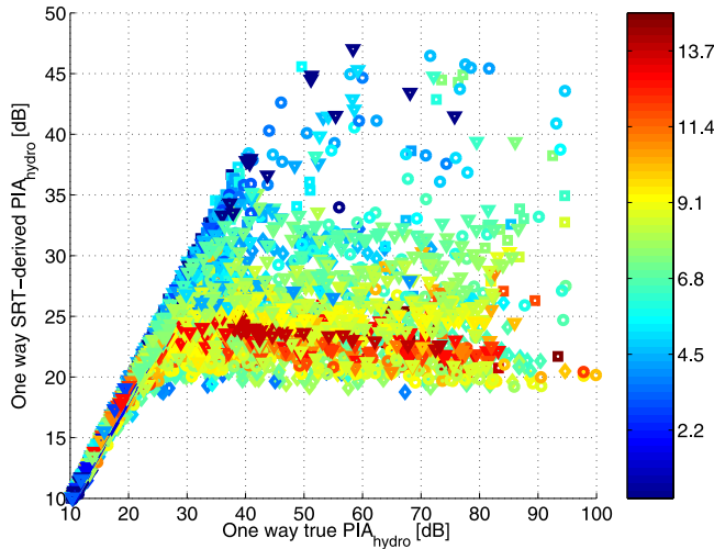
Figure 6. True one-way PIA_{hydro} versus one-way SRT-derived PIA_{hydro} . Diamonds, squares, circles, and triangles correspond to fronts, squall lines, extratropical storms, and hurricanes, respectively. The colorbar indicates the “10-dBZ height above the freezing level” in kilometers (see text for details).
