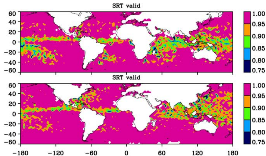
Figure 10. Global maps of the fraction of raining scenes during the period (top) from December 2006 to February 2007 and (bottom) from June 2006 to August 2006 in which the PIA can be correctly estimated by the SRT.
