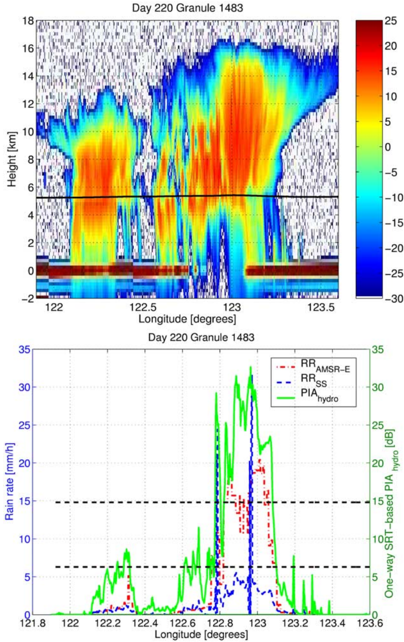
Figure 8. Case study for Tropical storm Bopha. (top) CPR reflectivities in dBZ; (bottom) estimated rain rates near surface from the SS-based CloudSat algorithm and from the collocated AMSR-E product and SRT-based estimated PIA.
