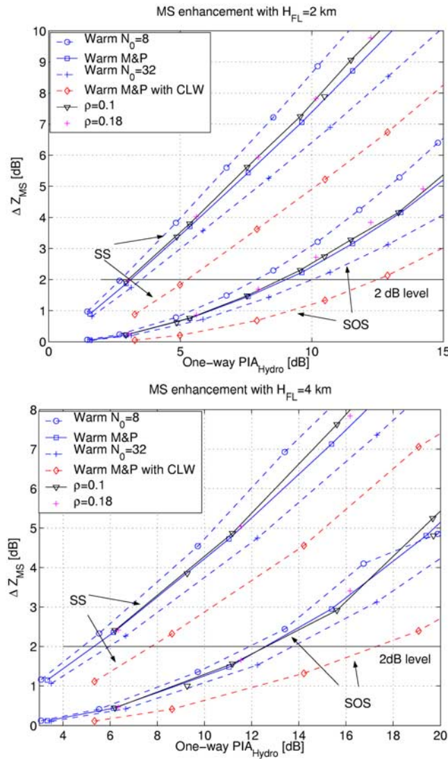
Figure 2. SSA and SOSA error in the return of the range gate close to the surface for vertical flux preserving scenarios with (top) H_{FL} = 2 km and (bottom) H_{FL} = 4 km. Two groups of curves are plotted: on the left/right side those relative to the SSA/SOSA error. Each group includes six different microphysics profiles as indicated in the legend (see text for details).
