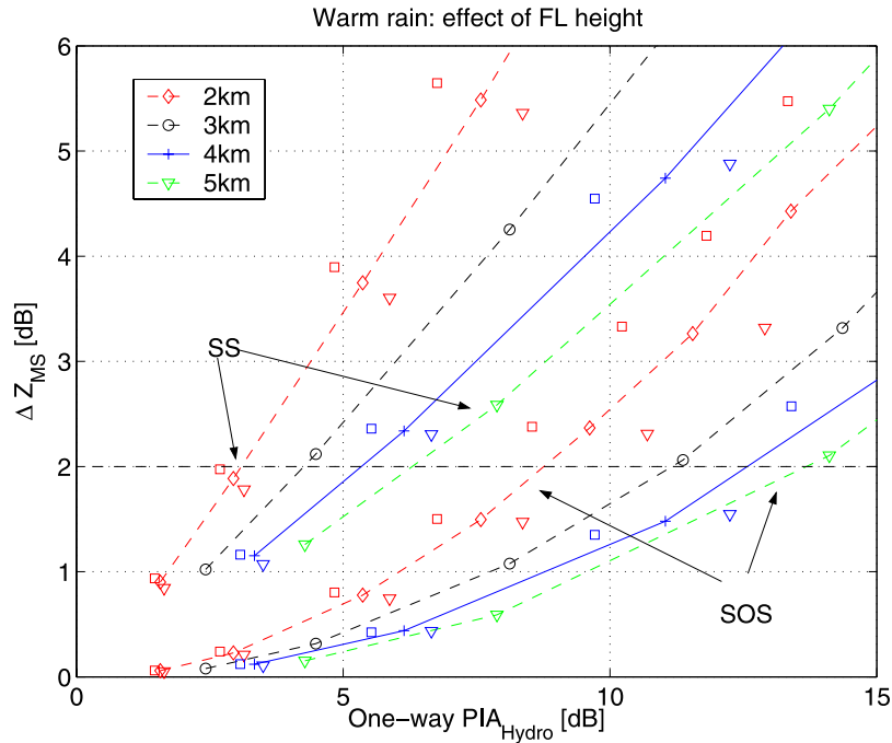
Figure 3. MS enhancement for warm rain with different freezing levels with N_0 = 8 \times 10^3 \text{ m}^{-3} \text{ mm}^{-1} as indicated in the legend. Two groups of curves are plotted: on the left/right side those relative to the SSA/SOSA error. In proximity of the curves corresponding to H_{FL} = 2 and 4 km the additional squares and triangles with the same grey scale represent cases with N_0 = 4, 16 \times 10^3 \text{ m}^{-3} \text{ mm}^{-1} , respectively.
