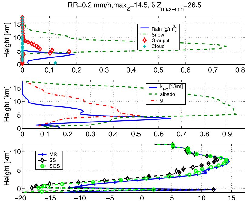
Figure 5. Example of an outlier extracted from Hurricane BOB CRM simulation.
