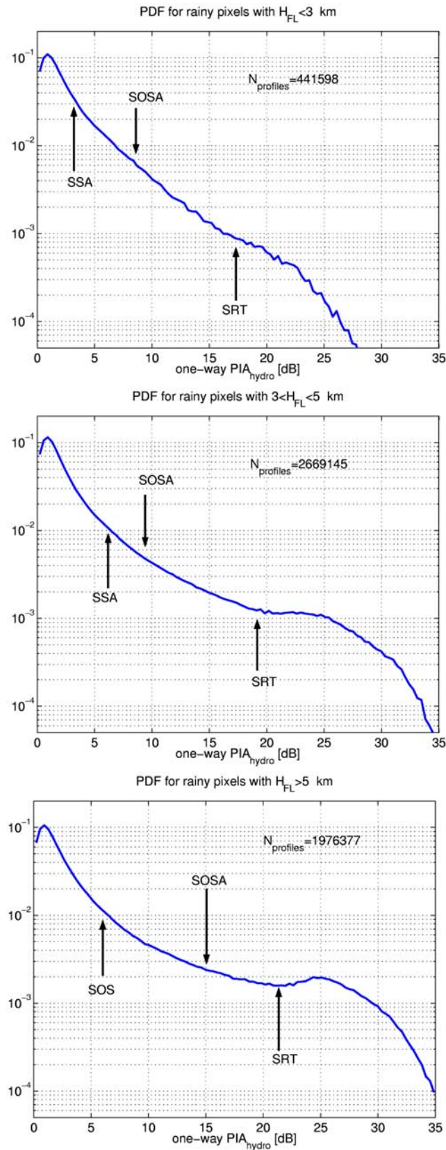
Figure 7. Probability distribution function of PIA hydro estimated by the SRT for rainy sea-surfaces pixels in the CloudSat database. The arrows indicate the 99% POD thresholds given in Table 1. The analysis covers the period from 15 June 2006 to 18 January 2007.
