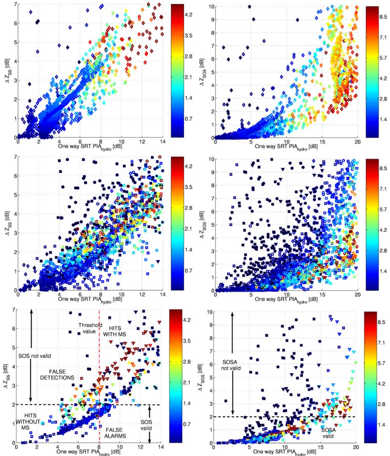
Figure 4. Enhancement of MS compared to (left) SSA and (right) SOSA as a function of the one-way hydrometeor PIA (estimated from SRT). The colorbar indicates the rain rate at the ground in mm/h. Diamonds, squares, circles, and triangles correspond to fronts, squall lines, extratropical storms, and hurricanes, respectively. Profiles have (top) FL < 3 km, (middle) 3 \text{ km} < FL < 5 km, and (bottom) FL > 5 km. Solid symbols correspond to profiles identified as “outliers” according to the criteria of equations (2)–(3). Profiles with \Delta Z_{SS} < 2 dB ( \Delta Z_{SOS} < 2 dB) may be treated with the SS (SOS) approximation.
