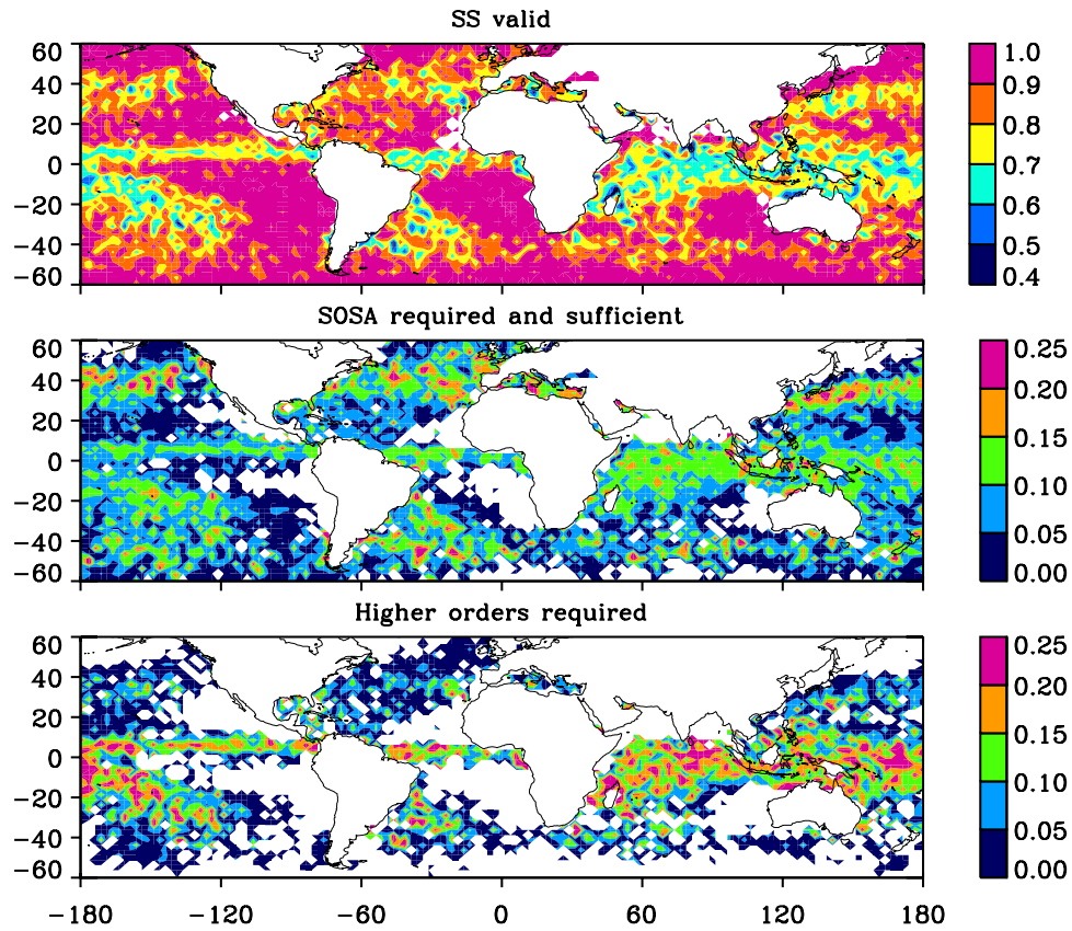
Figure 9. Global maps of the fraction of raining scenes during the period from December 2006 to February 2007 in which (top) the SS approximation is valid, (middle) the SOSA is required and sufficient, and (bottom) higher orders of scattering are required.
