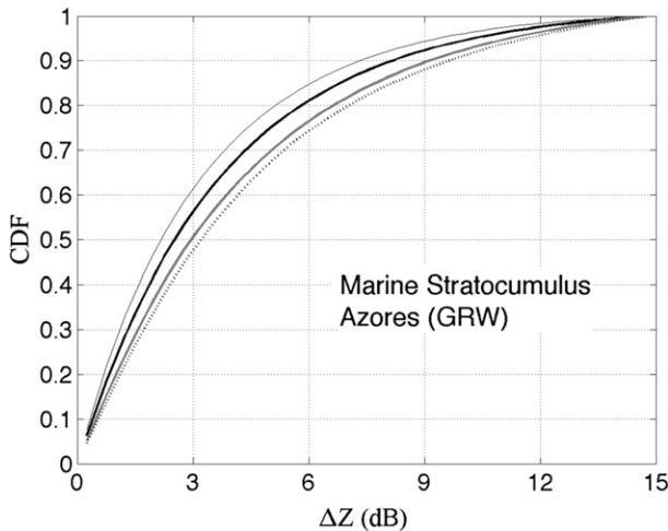
FIG. 7. Cumulative probability distributions function of observed \Delta Z for different horizontal lengths: 500 (thin gray), 1000 (thick black), 2500 (thick gray), and 5000m (dotted gray) in marine stratocumulus observed by the WACR during the AMF GRW deployment. Only WACR cloud detections in the lowest 2 km of the atmosphere and with high-cloud-fraction conditions (above 80%) have been used.
