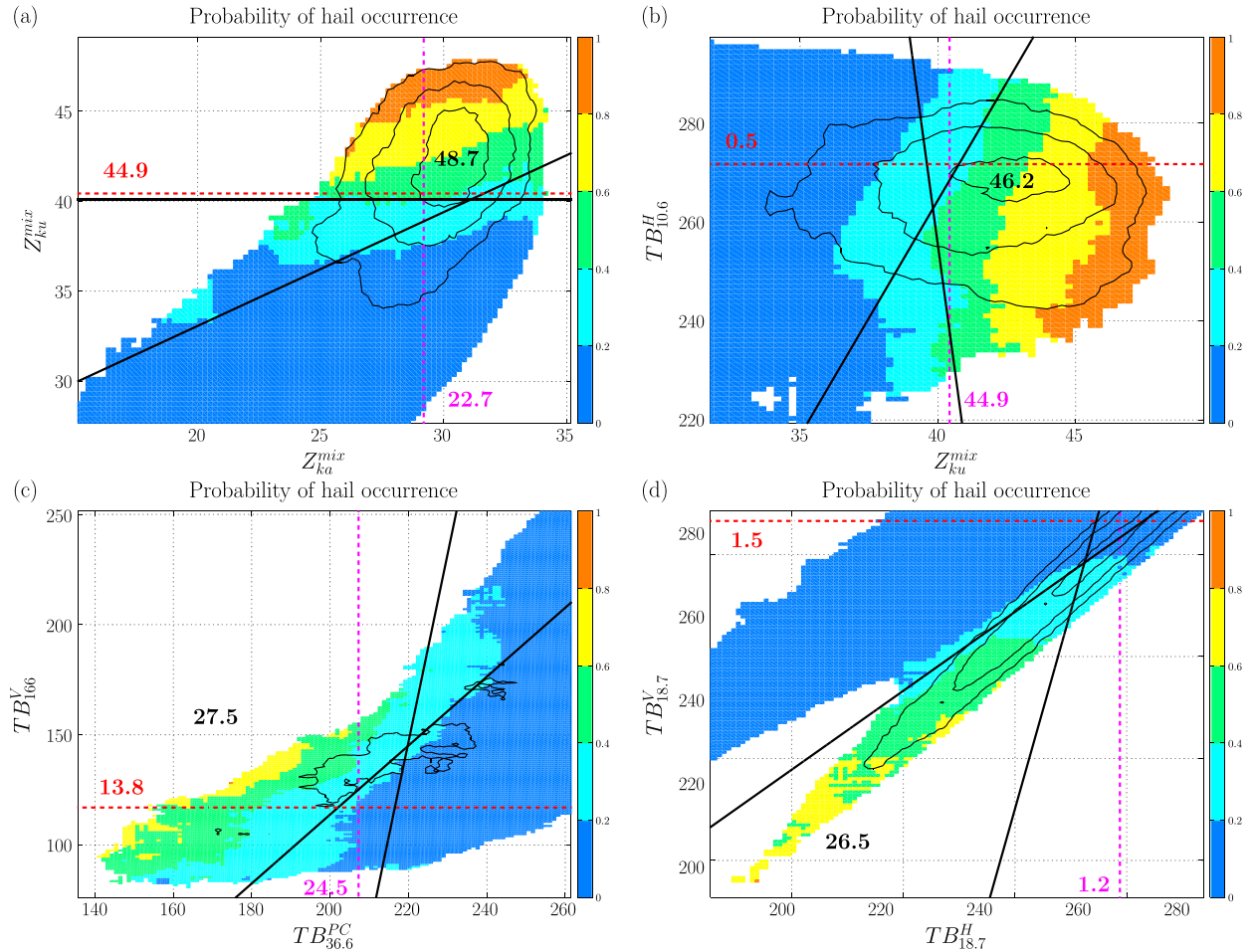
FIG. 5. The probability of hail occurrence depending on two parameters: (a) Z_{Ku}^{mix} and Z_{Ka}^{mix} , (b) Z_{Ku}^{mix} and TB_{10.6}^H , (c) TB_{36.6}^{PC} and TB_{166}^V , and (d) TB_{18.7}^H and TB_{18.7}^V . Thick black lines mark the boundary of the region that maximizes the CSI. Dashed lines mark the proxies in a single-parameter setting, and the numbers in the same color denote the CSI of each single-parameter proxy. Black numbers correspond to the CSI value of the dual-variable algorithm. Thin black contour lines show the domain of measurements associated with 2%, 5%, and 10% of all hail occurrences.
