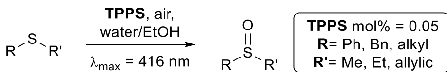
Figure 1: Typical reaction conditions for the sulfides oxidation.
