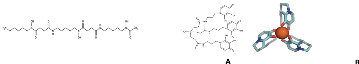
Figure 2: Structure formulae of DFO ( A ) and KC18 ( B ); molecular model of [Fe(KC18)] ( C )
