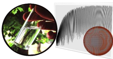
Figure 1: DES system and BZ's oscillation/chemical waves.
