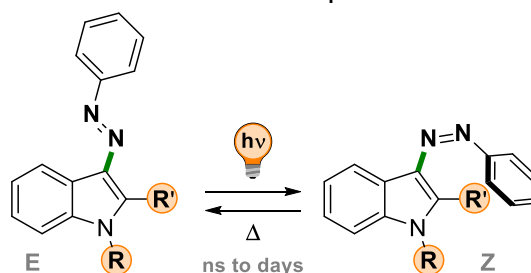
Figure 1: 3-phenylazoindole photoswitches.
