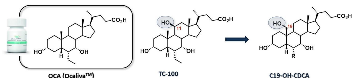
Figure 1: Structure of OCA, TC-100 and C19-OH-CDCA.
