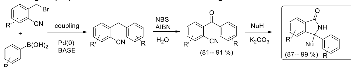
Figure 1: Reaction pathway.
