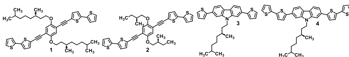
Figure 1: Chiral n-conjugated oligomers 1–4 studied in the present work.
