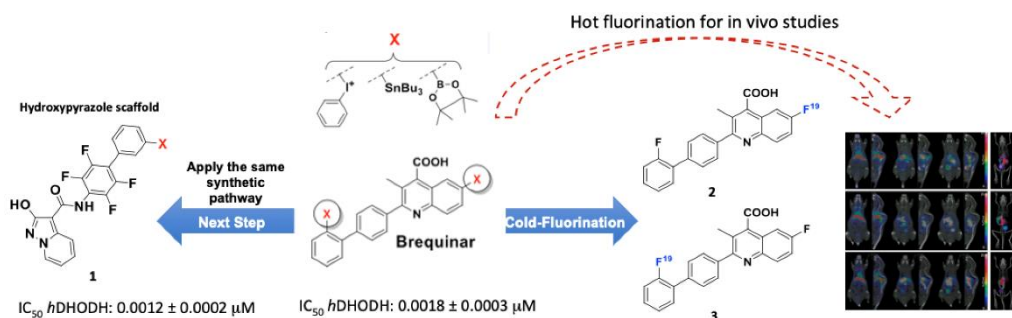
Figure 1: Design of novel hDHODH inhibitors probes.
