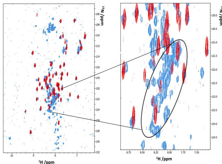
Figure 1: Overlay of 2D [ ^1\text{H} , ^{15}\text{N} ] HSQC spectra of ^{15}\text{N} , ^{13}\text{C} uniformly labeled Phox2b-HD (red) and Phox2b-Cter (20Ala) (blue).
