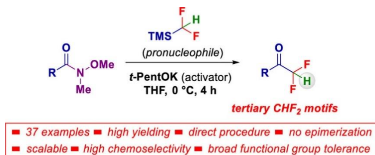
Figure 1: Reaction conditions.
