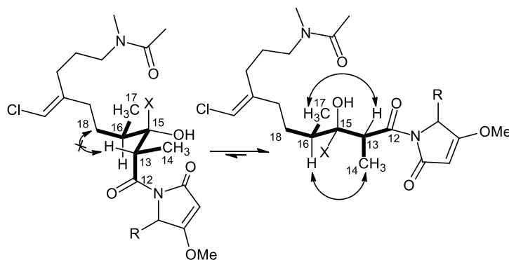
Figure 1: Determination of the relative and the absolute configuration at C-13, C-15, and C-16 of smenamide F and G.
