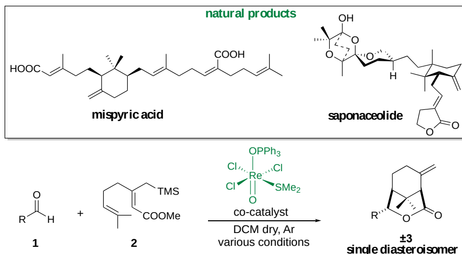
Figure 1: Synthetic targets and general reaction scheme.
