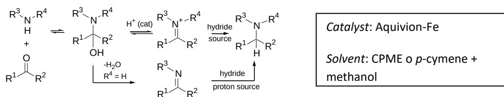
Figure 1: Reaction mechanism.
