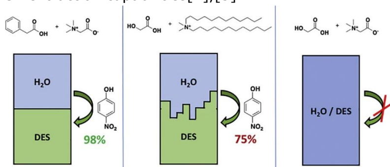
Figure 1: Extraction capabilities of novel Hydrophobic DESSs.
