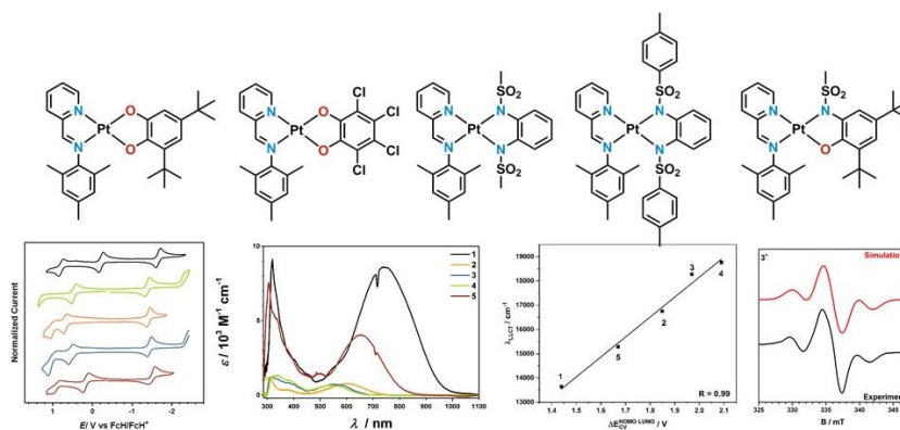
Figure 1: Investigated Pt(II) complexes and characterization.
