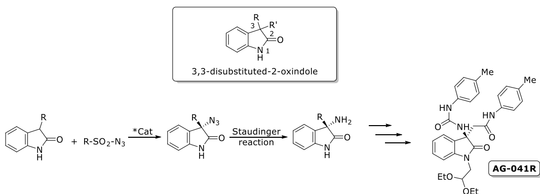
Scheme 1: Enantioselective organocatalyzed \alpha -azidation and elaboration in the bioactive compound AG-041R.
