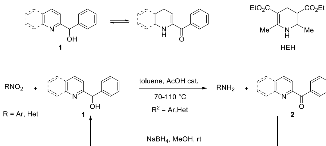
Scheme 1: Metal-free reduction of \text{RNO}_2 with compounds 1 .
