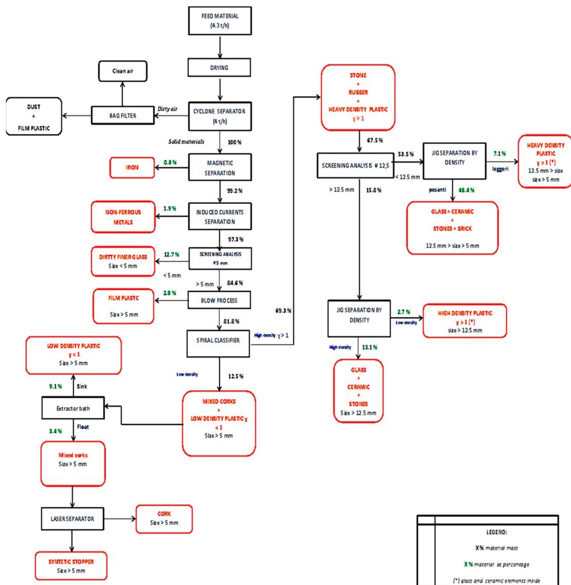
Figure 6. The new process plant suggested: apparatus and percentage of different materials obtained with the new plant.
