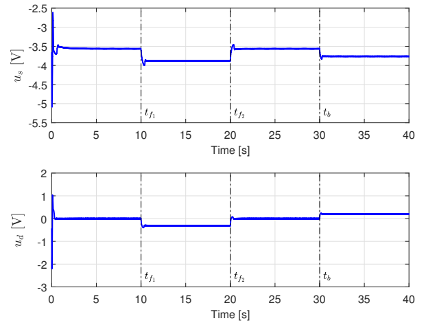
Fig. 4. Super-Twisting Controllers.
