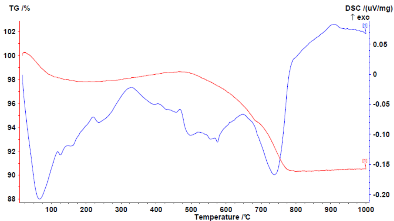
Figure 2. Thermogravimetric and differential thermogravimetric curves of the clay.
