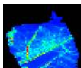
Figure IX.45. Left: SEM image of a hBN crystal flake. Right: Cathodoluminescence mapping of the D/S ratio of the integrated intensity of the D band relative to that of the S band. Adapted from [1048], © IOP Publishing Ltd.
