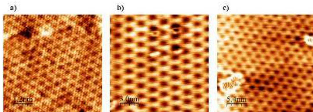
Figure V.28. STM images of SLG grown from \text{C}_{60} on: (a) Pt(111), ( 6 \times 6 ) nm, 0.11 V, 2.3 nA. (b) Ir(111), ( 15 \times 15 ) nm, 1.2 V, 2.6 pA and (c) Cu(111), ( 27 \times 27 ) nm, -0.4 V, 2.7 pA. In every image different moiré superstructures are shown.
