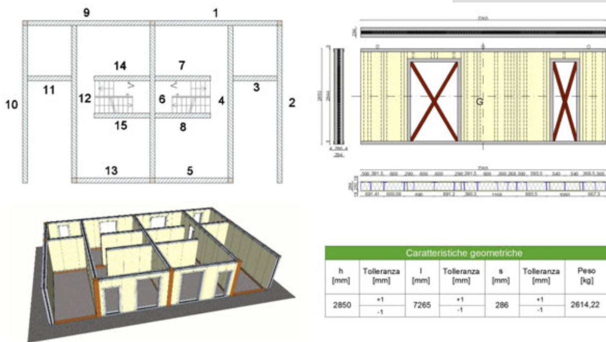
Figure 6. Example of panel subdivision - Example of reference panel technical data sheet.
