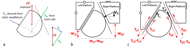
Figure 4: a Scheme representing the right contact force measurement and the derivation of the left contact force resultant. b Schematic of platform-to-platform hysteresis cycle relevant quantities. c Schematic of platform-to-damper (local) hysteresis cycle relevant quantities.
