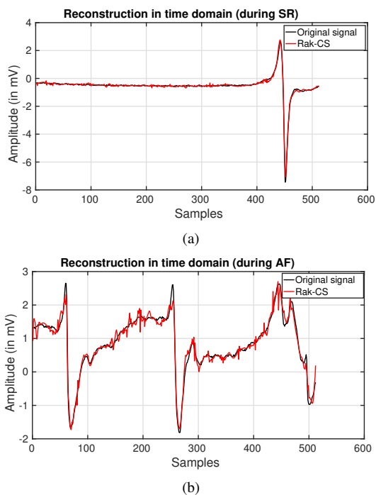
Fig. 6: Reconstruction of the time-domain waveform of atrial electrograms at CR = 4.26 (N=512): during (a) SR (b) AF.
