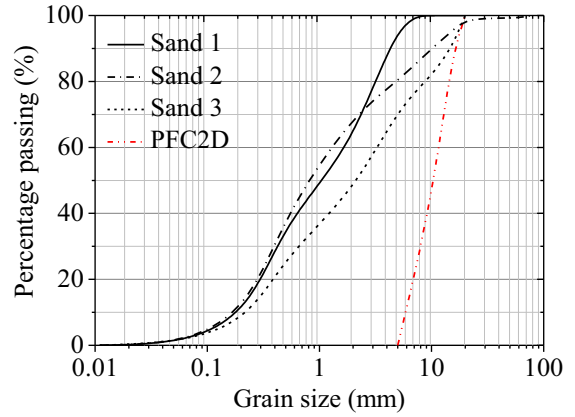
Fig. 2. Particle size distribution curves for sandy soils in the field and in the numerical model.
