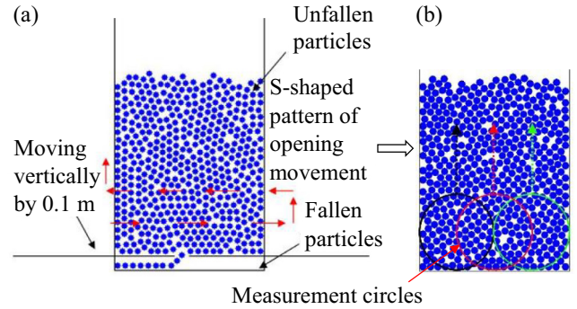
Fig. 4. Minimum packing using pluviation methods: (a) illustration of opening movement, and (b) measurement circles for density calculation.
