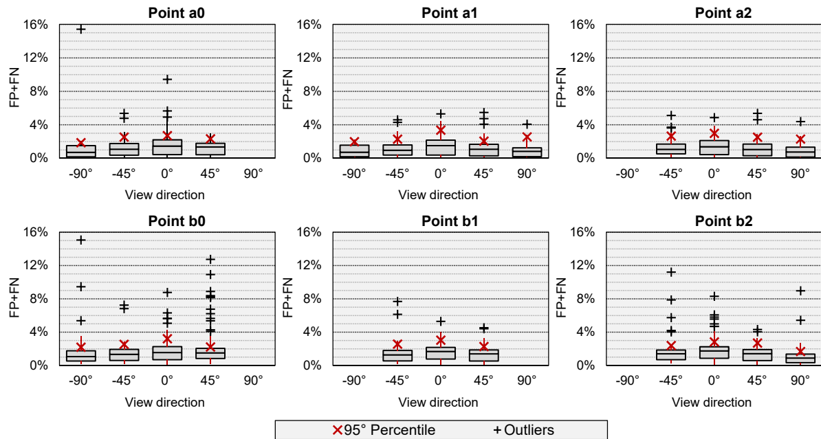
Figure 5 – Boxplots and 95 th percentile values relative to the error distributions (expressed as FP+FN), for each viewpoint and direction of view.
