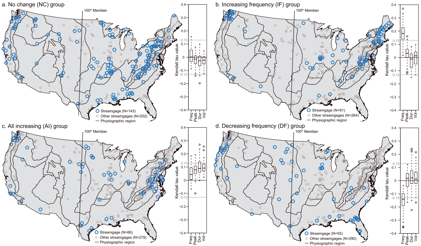
Figure 3. Streamgages experiencing similar changes in flood events. Streamgages clustered into one of four groups experiencing similar changes in the frequency (Freq), peak magnitude (Peak), duration (Dur), and volume (Vol) of flood events over the period 1940–2013 relative to a base period from 1940 to 1969 that averaged two flood events per year. Streamgages in (a) the no change (NC) group generally show no change in the flood properties; streamgages in (b) the increasing frequency (IF) group generally exhibit an increasing frequency of events; streamgages in (c) the all increasing group (AI) show increases across all flood properties; and streamgages in (d) the decreasing frequency (DF) group generally exhibit a decreasing frequency of events. Box plots of the Kendall tau values—a measure of relation between time and the flood properties—for the streamgages within each group is shown to the right of each map. A negative Kendall tau value indicates a decreasing trend; a positive value indicates an increasing trend. Correlations above values of 0.13 and below values of -0.13 (shown in grey lines) are generally significant correlations at a significance level of 0.1. Streamgages that are members of the respective cluster are shown as an open blue circle; streamgages that are part of the study but not a member of the cluster are shown as open gray circles.
