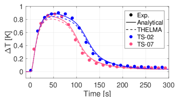
Fig. 6. Temperature increase evolution at TS07 (pink) and TS02 (blue) sensors for Shot #36-1: experimental (solid with circles) and computed results using 4C with analytical model (solid) and power input from THELMA (dashed).
