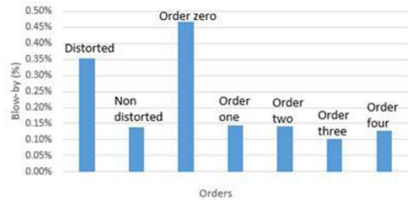
Fig. 23. Blow-by for different distortion orders.
