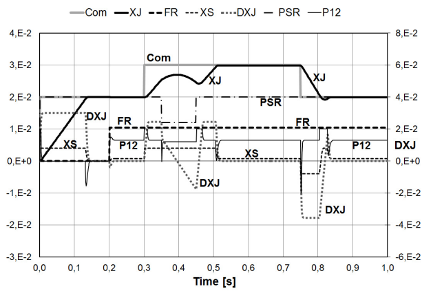
Figure 20. Dynamic response of the EHA model – MODEL C2
