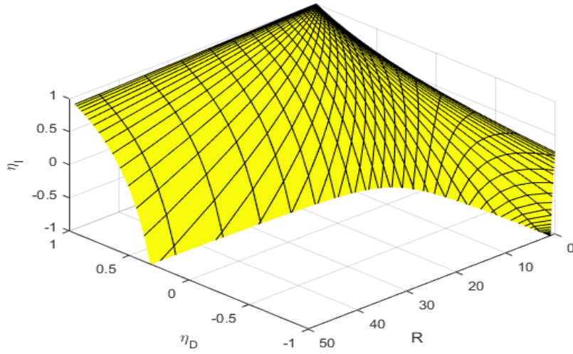
Figure 3 Surface plot of equation (14).
