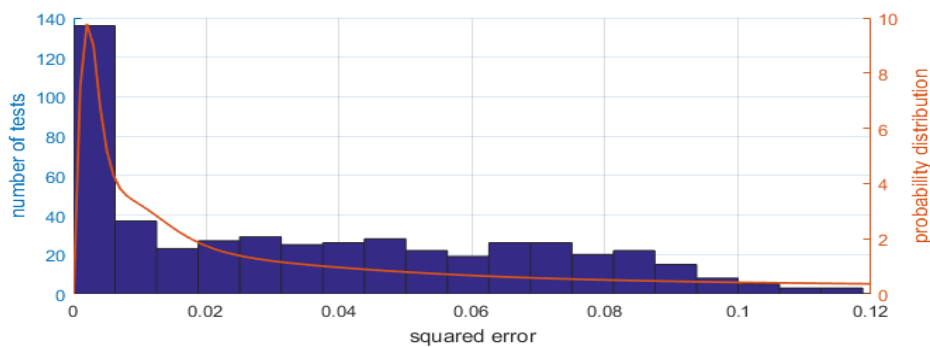
Figure 4 Distribution of the total squared error between the two models.
