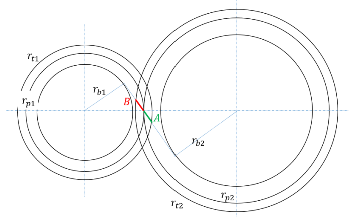
Figure 1 Reference gear geometry
