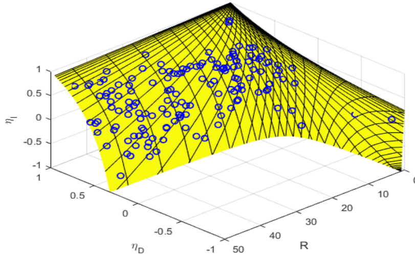
Figure 4 Comparison between the two models. The blue circles are the data points computed with the reference model.
