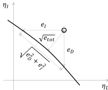
Figure 5 Graphical representation of the derivation of total error. The solid curve is the simplified model, the circle is the reference model data point.
