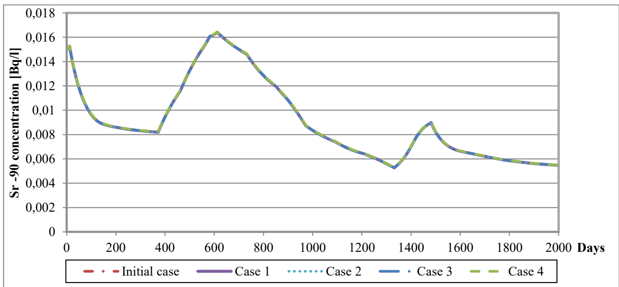
Figure 5 Sr-90 concentration in SP01 monitoring well for flow rates in Cavour channel equal to 14.67 \text{ m}^3/\text{s} (initial case), 7.33 \text{ m}^3/\text{s} (case 1), 1.47 \text{ m}^3/\text{s} (case 2), 44 \text{ m}^3/\text{s} (case 3), 146.67 \text{ m}^3/\text{s} (case 4).
