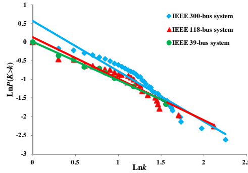
Fig. 3. Cumulative distributions of vertex degree in CFGs
