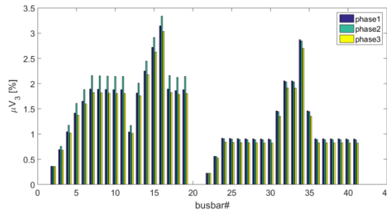
Figure 4. Mean value of the 3rd voltage harmonic at all busses
