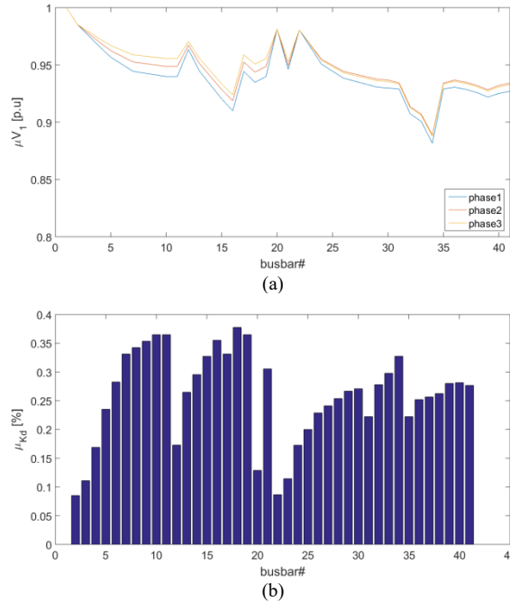
Figure 3. Mean value of the fundamental phase voltage (a) and mean value of the unbalance factor at all network busses (b)
