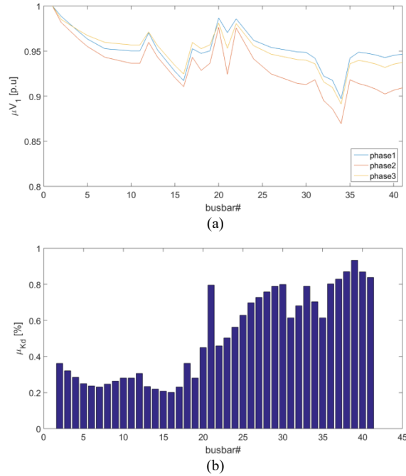
Figure 7. Mean value of the fundamental phase voltage (a) and of the mean value of the unbalance factor at all network busses (b)
