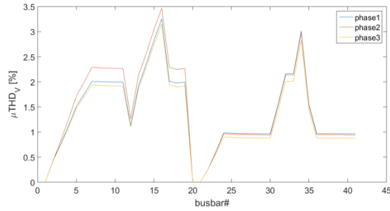
Figure 6. Mean value of the THD of voltage at all busbars
