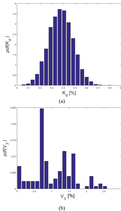
Figure 2. Probability density function of the unbalanced factor at bus #16 (a) and of the amplitude of the 3rd voltage harmonic at phase 2 of bus #15 (b)
