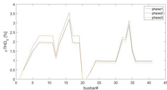
Figure 10. Mean value of the voltage THDv at all network buses.
