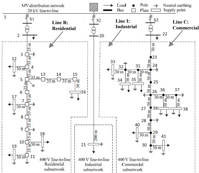
Figure 1. Cigré low voltage test grid [19]
