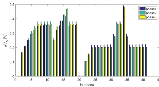
Figure 5. Mean value of the 5th voltage harmonic at all busses
