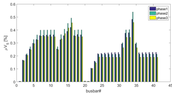
Figure 9. Mean value of the 5th voltage harmonic at all network buses
