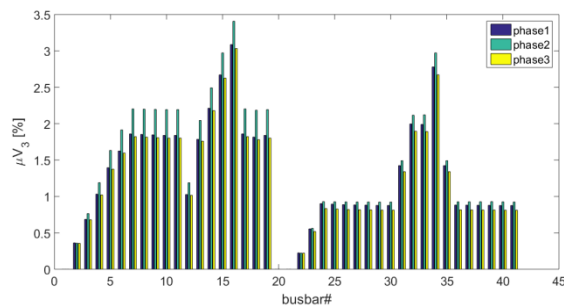
Figure 8. Mean value of the 3rd voltage harmonic at all network buses
