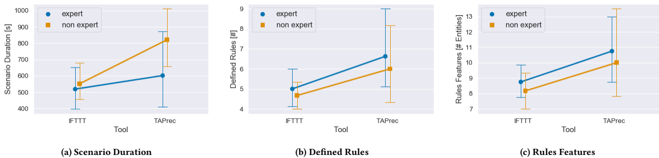
Figure 7: Independently of the participant groups, the usage of TAPrec increased (a) the time spent by the participants in personalizing a given scenario, (b) the total number of defined rules, and (c) the number of different connected entities involved in the define rules.
