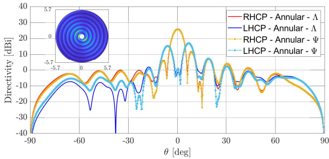
Fig. 7. Directivity of isotropic MS antenna similar to [8]: LHCP and RHCP radiated by the antenna for \theta \in [-90, 90] and \phi = 0 simulated with N_\Lambda = 195253 RWG and with N_\Psi = 908 Coaxial Entire-Domain Basis Functions.
