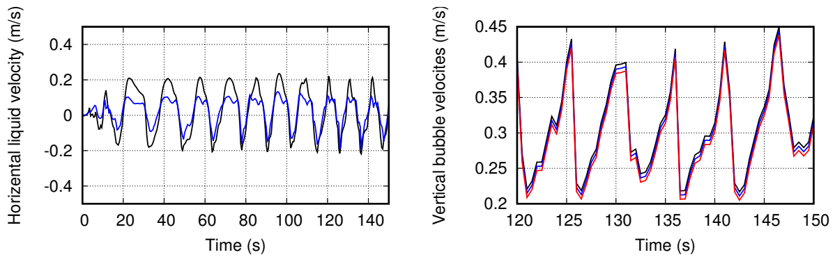
Figure 12: Left: The prediction of the horizontal liquid velocity by twoWayGPBEFoam at two different points (superficial velocity is 0.0024 m/s). Black line: x = 0.1 m, y = 0.225 m, z = 0.02 m. Blue line: x = 0.05 m, y = 0.225 m, z = 0.02 m. Right: the prediction of the vertical bubble velocities by twoWayGPBEFoam for small bubbles (black line), medium bubbles (blue line) and large bubbles (red line) at x = 0.1 m, y = 0.225 m, z = 0.02 m.
