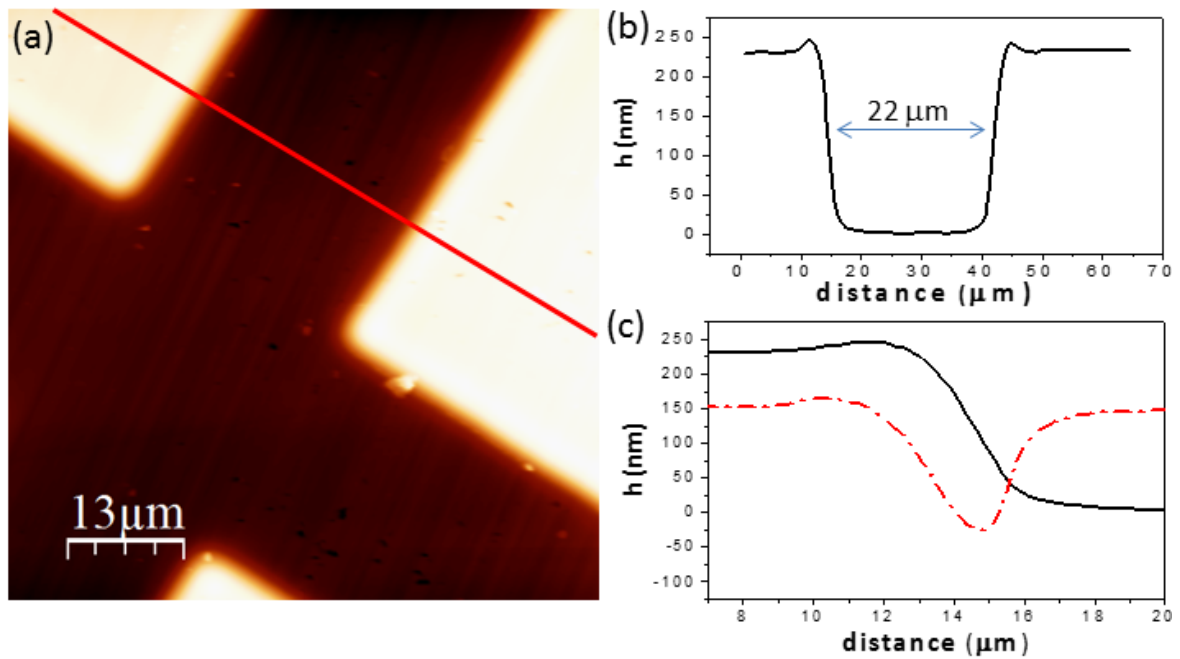
Fig. 2: a) Topography as measured by AFM of a diamond single-crystal sample after irradiation with a 10 MeV Au beam at a fluence of 5 \times 10^{14} \text{ cm}^{-2} . An 80 \text{ μm} -mesh mask with 60 \text{ μm} square apertures was used during irradiation. b) Profile along the segment indicated in the image in (a). c) Magnification of the step edge profile (black line) and its derivative (red dot-dashed line) to better visualize the abruptness of the step.
